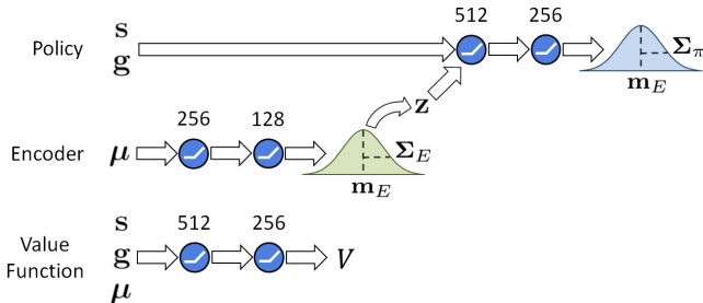
Fig. 6. Schematic illustration of the network architecture used for the adaptive policy. The encoder E(z|\mu) receives the dynamics parameters \mu as input, which are processed by two fully-connected layers with 256 and 128 ReLU units, and then mapped to a Gaussian distribution over the latent space Z with mean m_E(\mu) and standard deviation \Sigma_E(\mu) . An encoding z is sampled from the encoder distribution and provided to the policy \pi(a|s, g, \mu) as input, along with the state s and goal g . The policy is modeled with two layers of 512 and 256 units, followed by an output layer which specifies the mean m_\pi(s, g, z) of the action distribution. The standard deviation \Sigma_\pi of the action distribution is specified by a fixed diagonal matrix. The value function V(s, g, \mu) is modeled by a separate network with 512 and 256 hidden units.
