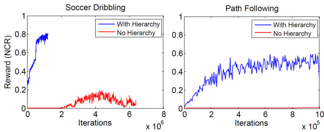
Fig. 11. Learning curves with and without control hierarchy.
