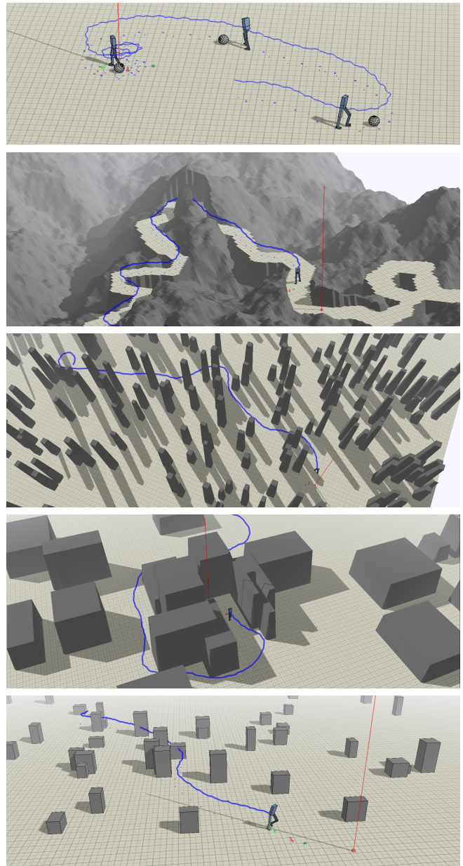
Fig. 12. Snapshots of HLC tasks. The red marker represents the target location and the blue line traces the trajectory of the character's center of mass. top-to-bottom : soccer dribbling, path following, pillar obstacles, block obstacles, dynamic obstacles.
