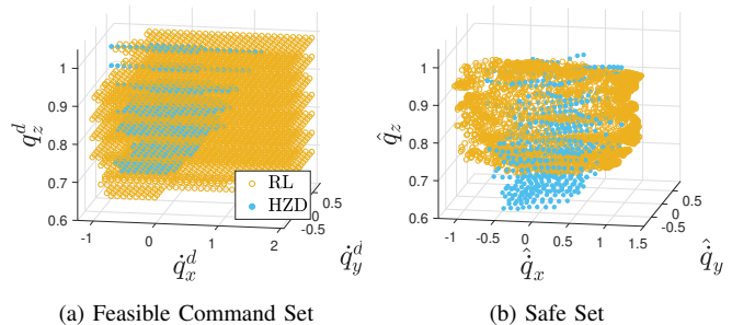
Fig. 4: Comparison of proposed commands (Feasible Command Set) and achieved commands (Safe Set) between HZD-based controller [17] and proposed RL-based controller. Our RL-based controller can handle more tracking commands than the HZD-based baseline and thus results in a larger feasible command set. The safe set of RL-based policy is also larger in the sagittal walking velocity \hat{q}_x and walking height \hat{q}_z direction. The tracking performance of the RL-based policy also shows advantages as the shapes of feasible command set and safe set are closer.
